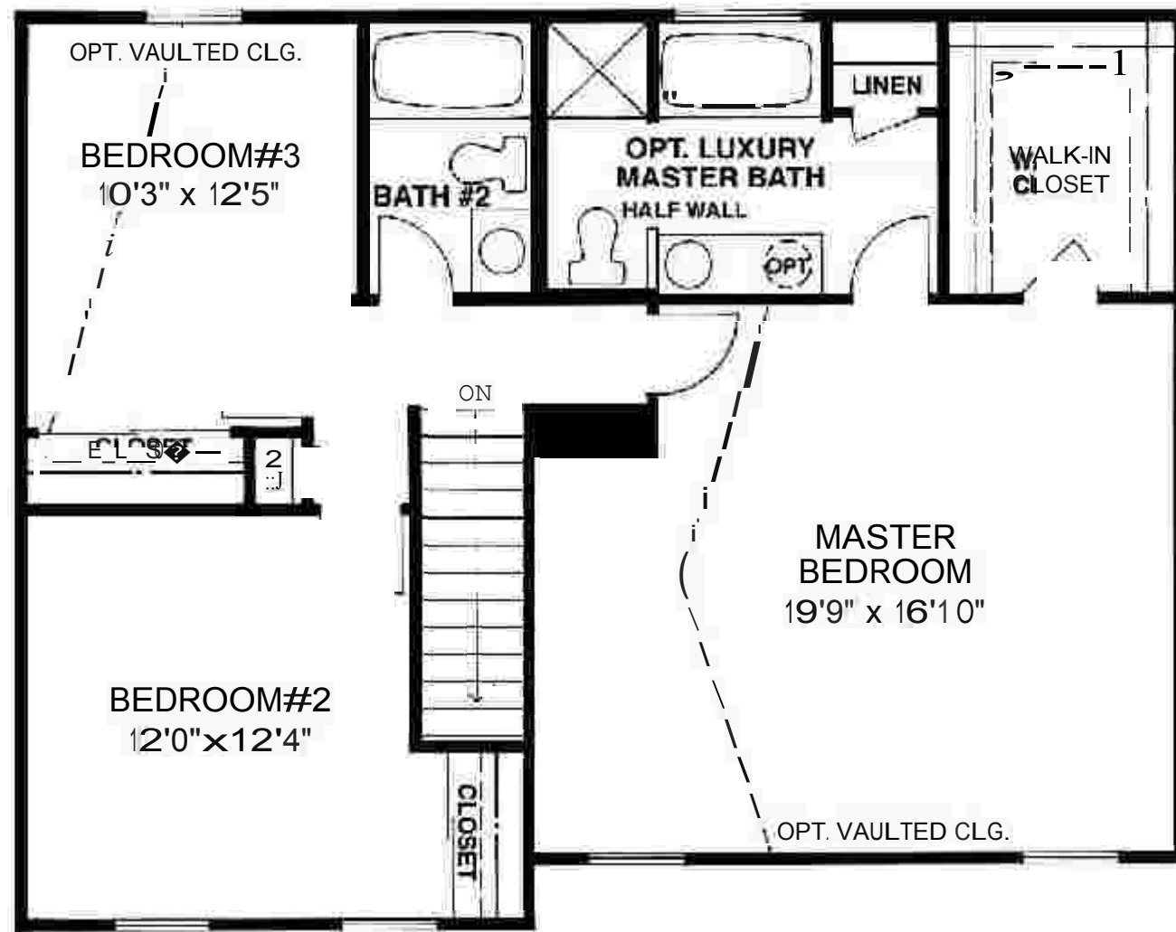
SECOND FLOOR PLAN - 3 BEDROOM
