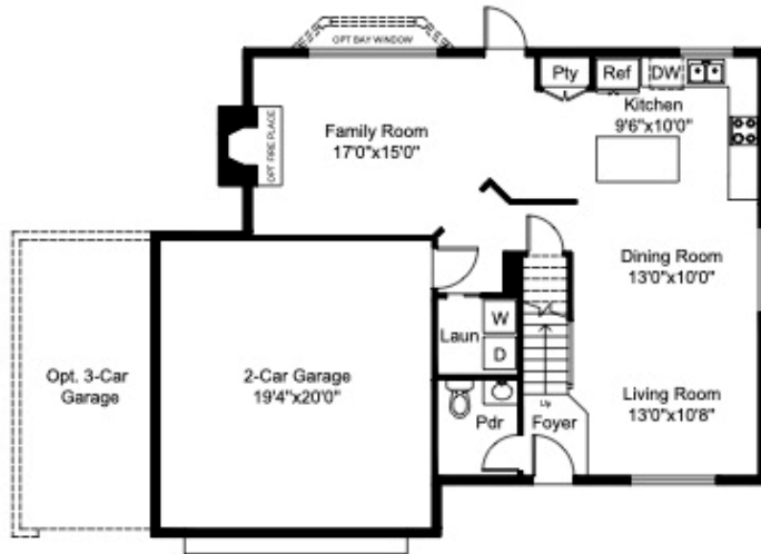
FLOOR PLAN PLAN
